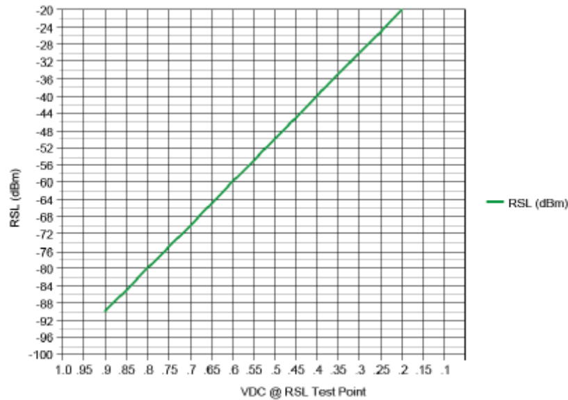
Figure 8 – Sample RSL Chart
